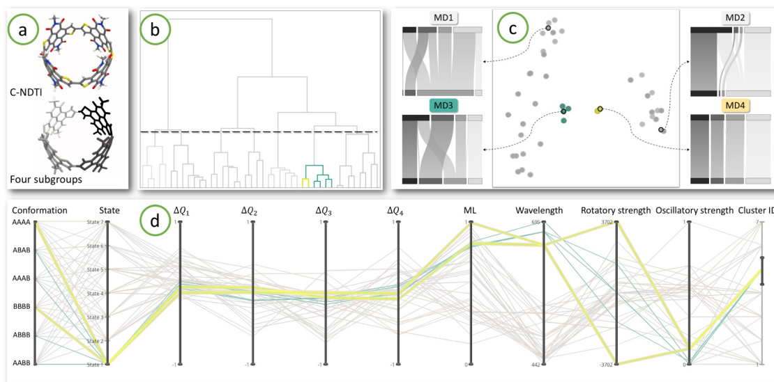
Figure 8: Finding correlations of charge transfer characteristics with the spectral properties of the transitions in the C-NDTI isomers ensemble. (a) The molecule consisting of four identical subgroups is shown. Each subgroup can have two orientations resulting in six different isomers which are explored in this study. (b) The dendrogram is shown along with a cluster highlighted in green which is different than other members of the ensemble in its charge transfer characteristics. (c) This is also evident from the 2D scatter plot as the green cluster lies in the middle while other points are distributed away and around it. Two points in this cluster appear separated from the other four and are highlighted in yellow. Four representative member transition diagram are shown selected from different regions. (d) Finally, the PCP is used for finding correlations with spectral properties of the transitions in this cluster. All members of the cluster belong to State 1 and have large wavelength. The two yellow transitions also have the highest absolute rotatory strength within the ensemble.
