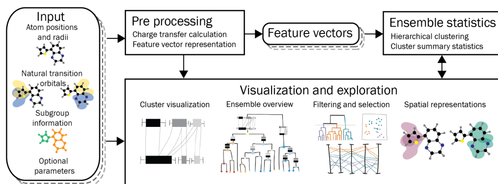
Figure 1: Pipeline for ensemble exploration of molecular electronic transitions: It takes an ensemble of simulations of molecule-light interactions as input, and combines automatic and explorative components to support an in-depth analysis.
