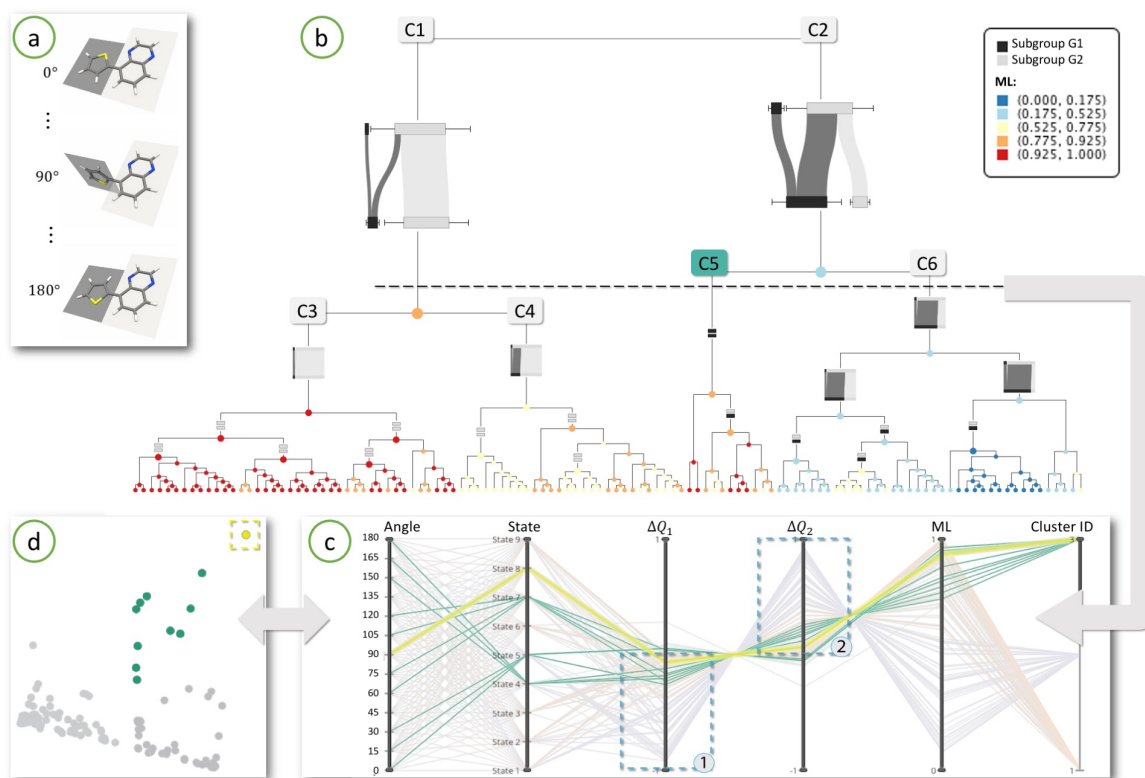
Figure 6: Top-down level of detail exploration of a Thiophene-Quinoxaline conformer ensemble using augmented dendrogram. (a) The molecule is composed of two groups, here available in 13 different conformations with dihedral angles varying from 0^\circ to 180^\circ . (b) The augmented dendrogram for the 117 transitions within this ensemble. Notice how the transitions group into two bigger clusters, each exhibiting different charge transfer characteristics. (c) The parallel coordinates plot shows an overview of the complete ensemble and highlights cluster C5 which is of interest. (d) The projection of ensemble in 2D using PCA. One outlier is identified using this scatter plot, highlighted in yellow.
