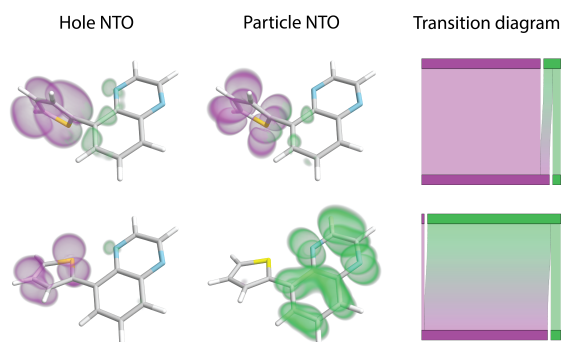
Figure 2: Spatial representations and member transition diagram for two transitions in a molecule with two subgroups, G1 (purple) and G2 (green). Top: LE type transition where the charge stays on the G1 . Bottom: CT type transition showing strong transfer from G1 to G2 . These transitions belong to the ensemble studied in Sec 7.1
