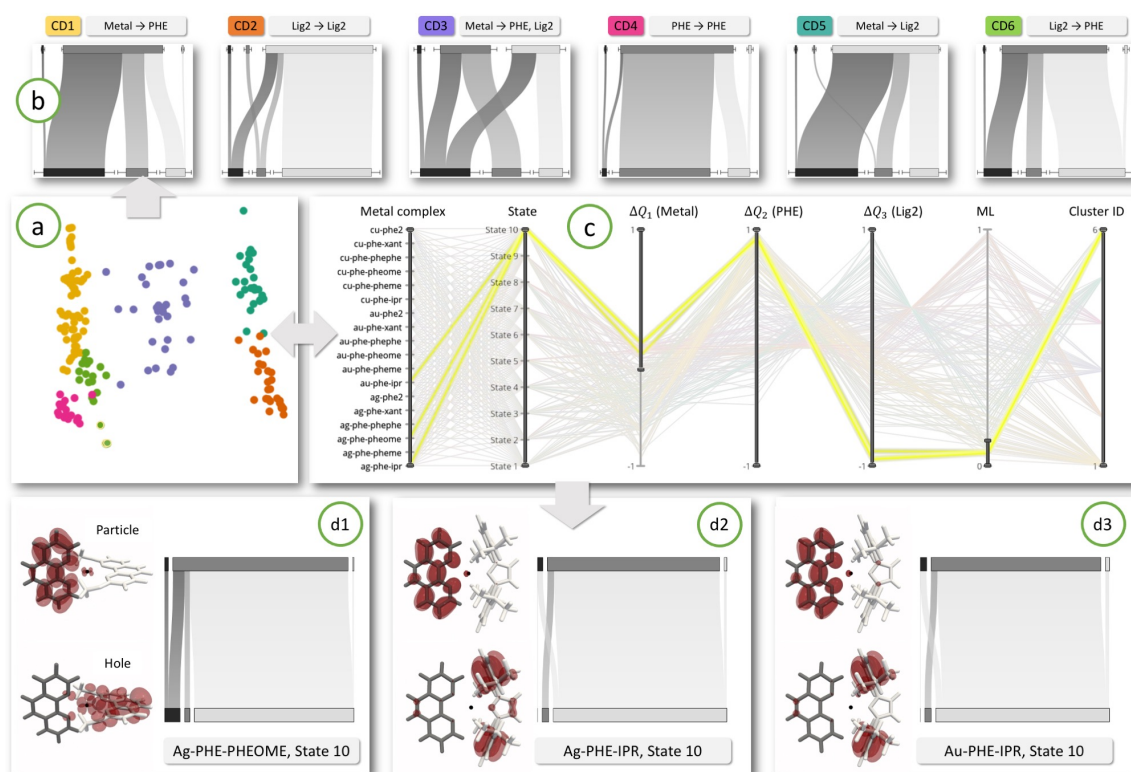
Figure 7: Using CDs to explore the nature of transitions in metal complexes consisting of a metal atom surrounded by two ligands (PHE and Lig2). (a) 2D projection of all the transitions in the ensemble, colored according to six identified clusters. (b) CDs for the six clusters, with subgroup order from left to right: metal, PHE, Lig2. Note the clear differences in charge transfer characteristics of the transitions in these clusters, and how the CDs convey this concisely and effectively. (c) Exploring the charge transfer character shown by CD6 in more detail, filtering the PCP reveals three similar transitions. (d1–d3) The spatial data from which the transitions were computed confirms our findings.
