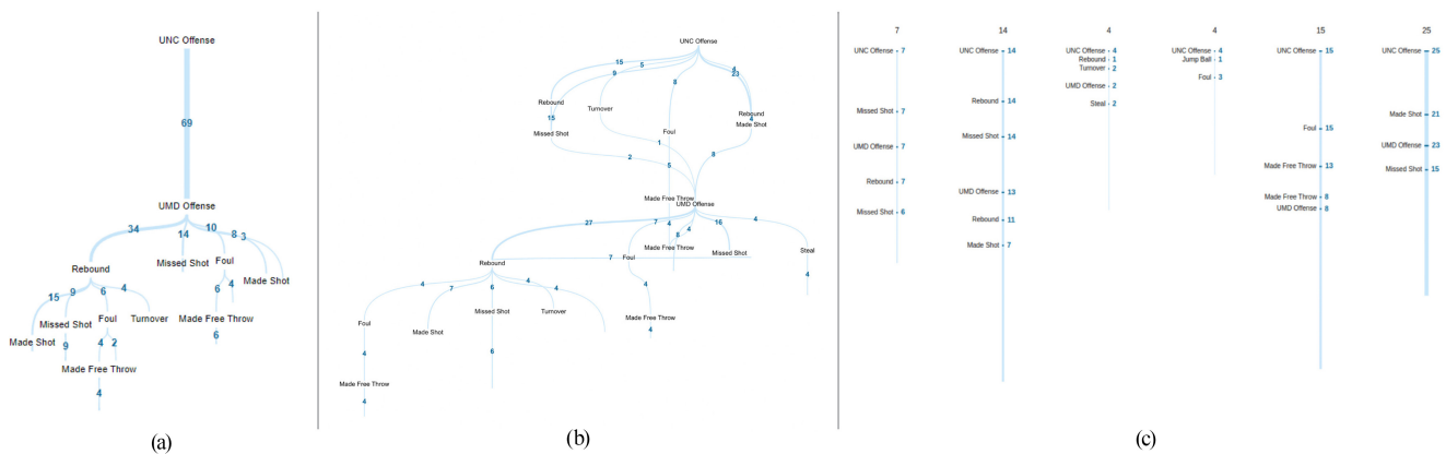
Figure 1: In our study, we generated visual summaries of the same dataset using three different techniques: (a) CoreFlow [LKD*17], (b) SentenTree [HWS17], and (c) Sequence Synopsis [CXR18]. These visual summaries were shown one at a time, and the participants were asked to rate how closely the visualization depicted given insights about the dataset and provide a justification for their ratings.
