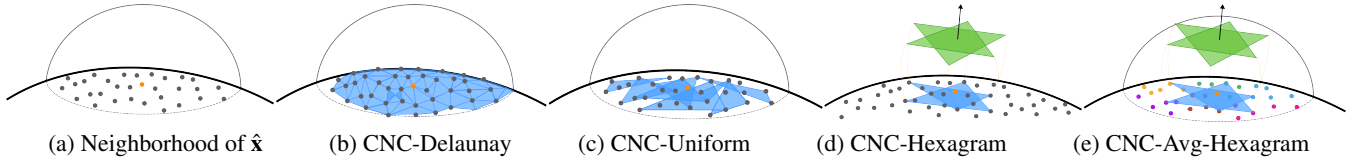
Figure 3: This figure illustrates the different strategies for generating the random triangles around the point of interest (see text).
