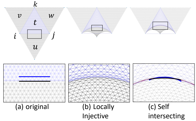
Figure 10: Example of a non-locally-injective transformation. (a): original triangles with part of e_{ij} in black and a parallel line inside t in blue. (b): an extreme deformation with matrix M of the bottom triangle u (while the rest are stationary) leads to edge ratios \delta_{ut} = M, \delta_{vt} = \delta_{wt} = Id . However, the result is still locally injective. By the barycentric blending, any line originally parallel to e_{ij} in t is transformed by matrices M^d , with varying d < \frac{1}{2} , and thus closer to Id than the transformation M^{\frac{1}{2}} of e_{ij} . In this case, e_{ij} would be more curved inwards than the other parallel lines within. Thus, in (c), when M is made even more extreme, the target black circular arc from edge e_{ij} and the less-curved blue curve transformed by M^d intersect, causing a loss of injectivity.
