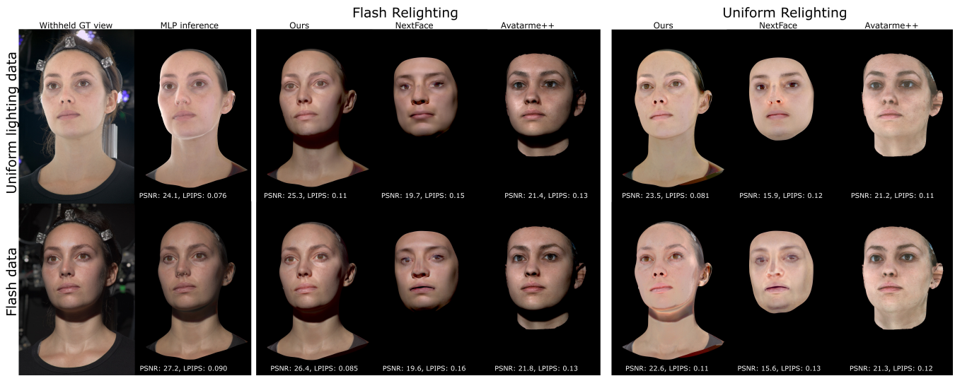
Figure 9: Quantitative comparison on Digital Emily [The15]. Each row showcases renderings created using results from the respective input capture (left) and the errors are computed against the respective ground truth observation, across the face area.
