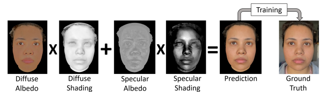
Figure 4: Rendering model: During training, the predicted diffuse and specular shading components are respectively multiplied by the albedos, then summed to produce the predicted rendering, which is supervised by the input images. The specular shading is additionally multiplied by a Fresnel term.
