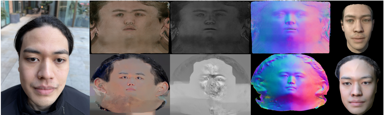
Figure 5: Left to right: Input image, diffuse albedo, specular albedo, specular normal textures, Blender rendering in novel lighting. Top: AvatarMe++ [LMP*21]. Bottom: Ours. Although more complete, the AvatarMe++ textures contain some inpainting artifacts (merged eye-brows) and missing details (cheek moles). Our method also preserves the skin tone and eye color more accurately.
