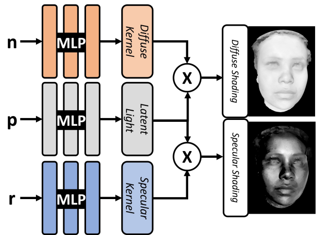
Figure 2: Three separate MLPs respectively learn spatially-varying lighting, a diffuse and a specular reflectance kernel, parameterized on world-space position \mathbf{p} , normal \mathbf{n} and reflected direction \mathbf{r} . View-dependent and -independent shading components are obtained via dot-product of kernels and lighting.
