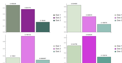
Figure 5: The feature visibility [WZC*11] histogram at top-left shows the sum of visibility values of all the voxels belong to each feature. The two histograms of visibility-weighted feature saliency from brightness and saturation respectively (at top-right and at bottom-left) show the sum of visibility-weighted saliency of all the voxels belong to each feature ( W_F(O, i, \sigma) in Section 3.3). The histogram of weighted feature saliency (at bottom-right) shows the weighted feature saliency with equal weights of brightness and saturation ( W_F in Section 3.4). Feature visibility (top-left) and visibility-weighted feature saliency from brightness (top-right) both suggest that the top disk is the most visible and the bottom disk is the least visible. However, the middle disk with magenta color is significantly more salient than the other two disks (light green and dark green) in terms of saturation (the histogram at bottom-left).
