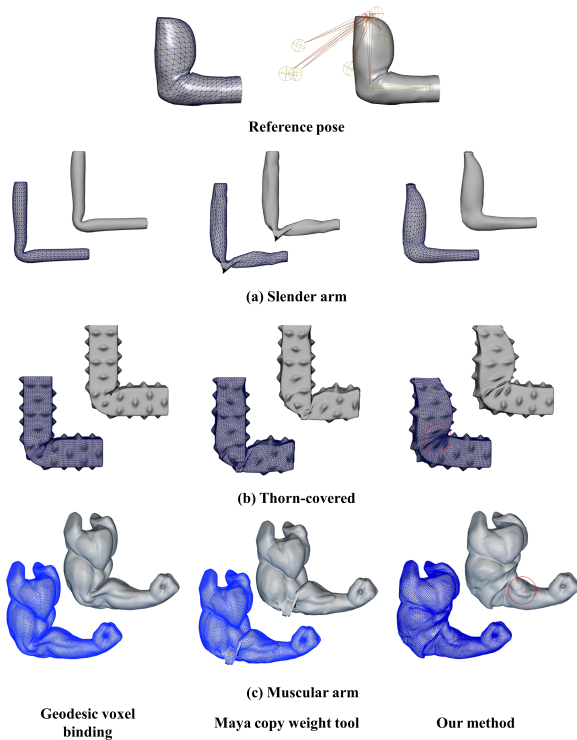
Figure 4: Experimental results of the arm models.
