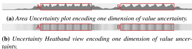
Figure 3: Visualization designs for showing value uncertainty. When using (a) Area Uncertainty plots, value uncertainties from different sources can be stacked. An alternative visual encoding is the (b) Uncertainty Heatband plot. The two marked areas (A, B) show areas where value uncertainty is introduced periodically.
