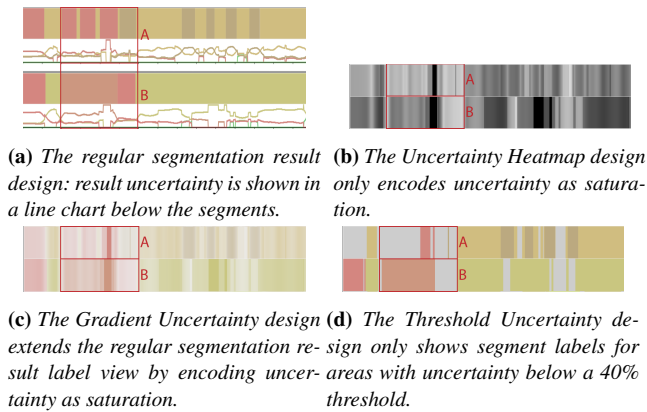
Figure 2: Visualization designs showing result uncertainty for uncertainty-aware segmentation result overview: the highlighted areas (A,B) show how time intervals were segmented by varying parameter settings and introduced uncertainty differently.
