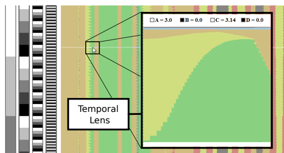
Figure 5: A temporal lens that magnifies a segment boundary near the mouse cursor and shows the exact temporal change of label probabilities as a stacked area plot.
