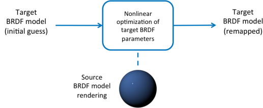
Figure 2: BRDF remapping scheme.
