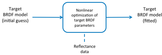
Figure 1: Basic scheme for BRDF fitting.
