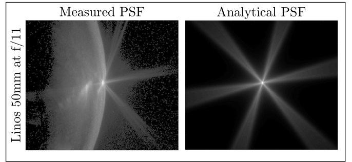
Figure 3: Comparison of the PSF resulting from the fitted diaphragm against a real HDR photograph of a quasi-point light source. Some slight differences can be observed in the repartition of light within the widened star branches of the PSF, which is explained by the random variations along the diaphragm edges that we do not take into account.
