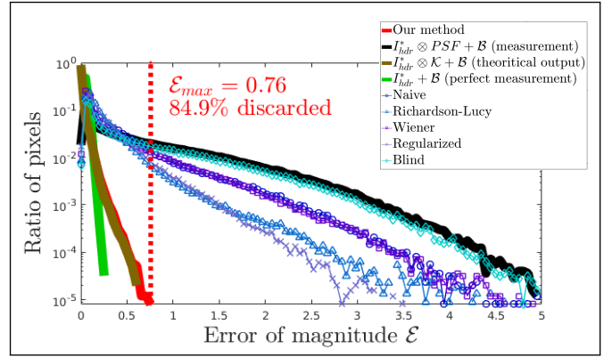
Figure 5: Histograms of the error of magnitude against a virtual reference (SNR=10) of the remaining valid pixels for different methods. The histogram of our method (red curve) is much more concentrated on the small errors than every deconvolution algorithm (blue curves). Of course, the quality of the original image (green curve) is not reached because of the residual kernel contribution, but our output error matches very well with the achieved output (brown curve) prediction.
