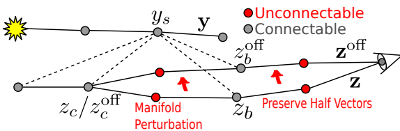
Figure 5: G-BDPT paths.
