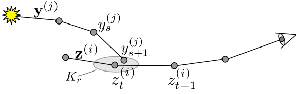
Figure 4: VCM paths.
