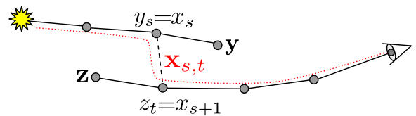
Figure 3: BDPT Paths.
