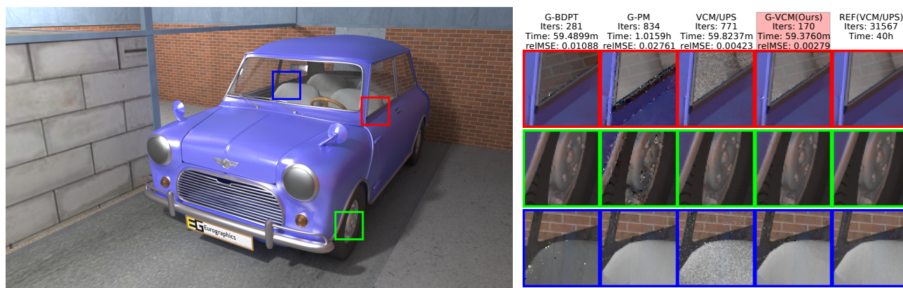
Figure 1: Equal time (1 hr) comparison in the Car scene. Here, G-BDPT iterations correspond to samples per pixel. Our method significantly reduces noise compared to VCM/UPS [GKDS12, HPJ12]. G-BDPT [MKA*15] completely misses the SDS path contribution on the seats and G-PM [HGNH17] struggles with the glossy window frame and wheel hub. Our method robustly captures all of these transport contributions.
