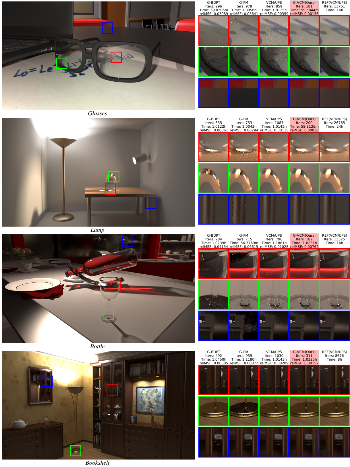
Figure 15: Equal time comparison between our method, G-BDPT, G-PM and VCM with L1 reconstruction for all gradient domain methods.
