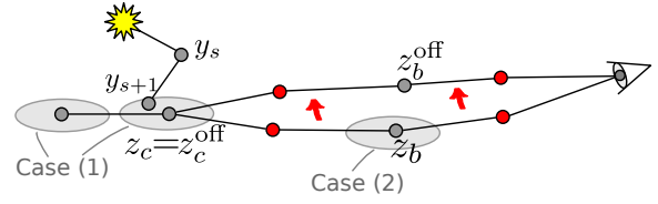
Figure 6: Gradient-domain vertex merging cases.
