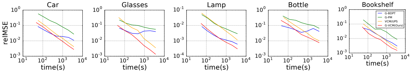
Figure 11: Error ( relMSE ) plots of all 5 test scenes, comparing G-BDPT , G-PM , G-VCM using L1 reconstruction and VCM .
