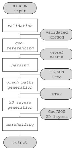
Figure 10: HIJSON Toolkit processing pipeline.
