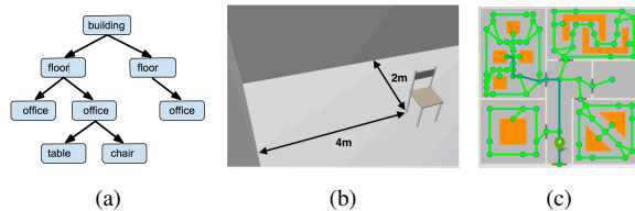
Figure 14: HIJSON + FIVE: (a) Hierarchical structures; (b) metric positioning of furniture e/o IoT devices in the local coordinate frame; (c) automatic construction of the whole graph of paths within the building.
