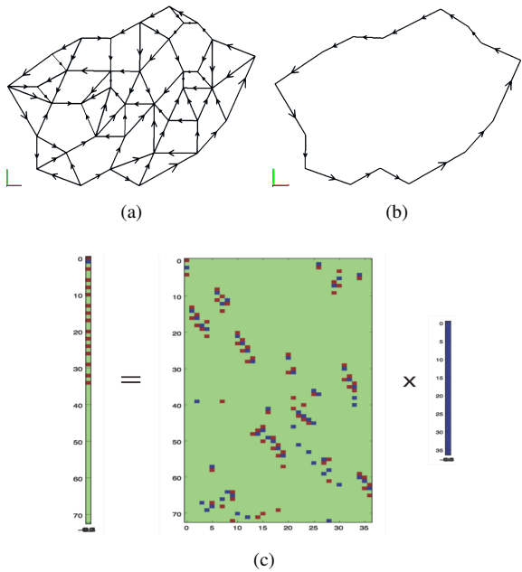
Figure 5: A toy example of the LAR scheme: (a) the bare minimum of data with complete information about topology; (b) the extracted boundary; (c) the extraction method [e] = [\partial][f] giving the coordinate representation (in the discrete basis of the 1-cells) of the boundary edges [e] by product of the sparse boundary operator matrix [\partial] times the coordinate representation [f] of the 2-cells (faces), in the discrete basis of the 2-cells.
