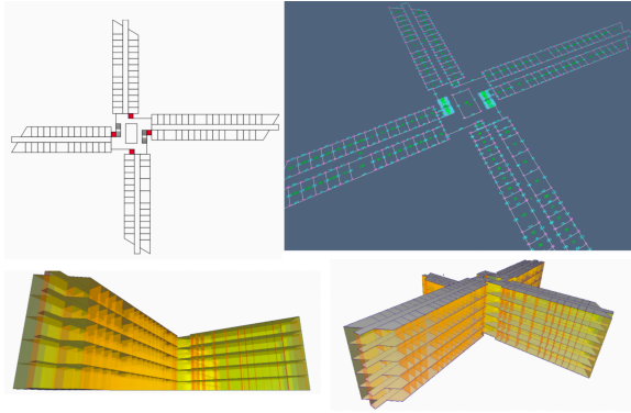
Figure 3: Office building: (a) the schematic plan —made of SVG primitives: lines, rects, polygons— possibly obtained via a client UI loading engineering design in background; (b) the automatically generated LAR cellular complex, transformed server-side into HIJSON; (c and d) the mock-up for the automatically generated 3D HIJSON.
