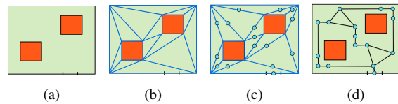
Figure 11: graph of paths generation: (a) detection of obstacles and computation of walkable area; (b) triangulation of walkable area; (c) identification of graph nodes; (d) junction of nodes.
