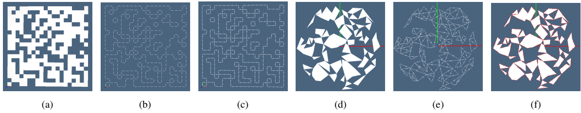
Figure 4: LAR examples: (a) 2-chain of quad cells; (b) boundary 1-chain; (c) oriented boundary; (d) random 2-complex; (e) oriented 1-skeleton; (f) oriented boundary (in red).
