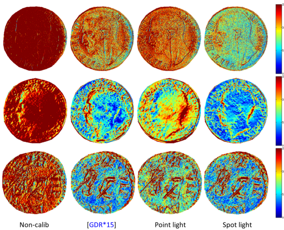
Figure 6: Normal map errors. Difference between PS estimated normals from the reference microprofilometer normals.
