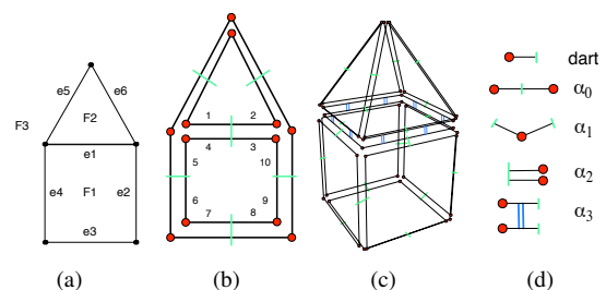
Figure 1: n -Gmap representations. (a) A 2D object containing 3 faces, 6 edges and 5 vertices. (b) Corresponding 2-Gmap: the set of darts \{1,2,3,4\} represents edge e_1 , the set of darts \{3,4,5,6,7,8,9,10\} represents face F_1 . (c) 3D object composed of 2 volumes represented with 3-Gmap. (d) Symbolic representation of involutions.
