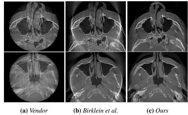
Figure 5: Slices of two different motion-impaired clinical CBCT acquisitions. Top row shows the reconstruction of a short scan (186°), bottom row a full scan.
