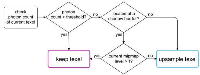
Figure 5: Multi-resolution image-filtering workflow.
