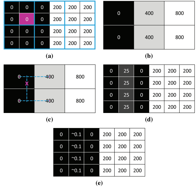
Figure 6: Four texels framed in blue (a) are summed up to one texel on the next higher mipmap level (b). A bilinear interpolation (c) near a shadow border can produce intensity leaks (d). Bilinear interpolation produces significantly smaller intensity leaks (e).
