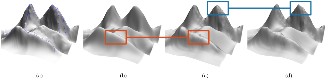
Figure 4: Structure-aware filtering: (a) terrain model with crest lines (indicated in blue); (b) filtering of the terrain using a uniform Gaussian filter kernel results in inappropriate flattening, here we use a size which is the maximal size of our structure-aware filter; (c) structure aware filtering with the Savitzky-Golay filter; (d) with our modified Gaussian filter, parts with a small distance to a crest line remain well in their elevation, while other details are smoothed (cf. boxes).
