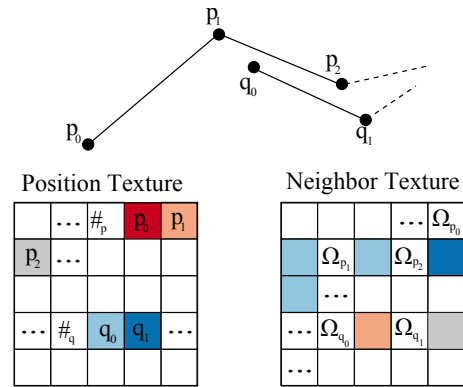
Figure 10: Streamline data texture for GPU-based neighbor selection. The vertex positions are mapped to a position texture and a neighbor texture. This allows us to retrieve neighboring information between strokes directly on the GPU.
