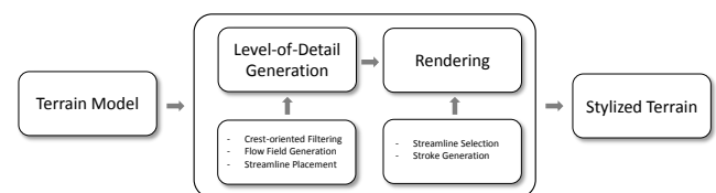
Figure 3: System Overview. In a preprocessing step we produce different Levels-of-Detail for a given input terrain. Here, we use crest-oriented filtering to smooth the terrain levels. A flow field is generated for each level and streamlines are placed. In the rendering step, streamlines are selected based on the LoD and strokes are generated depending on the underlying terrain type to produce a stylized model.
