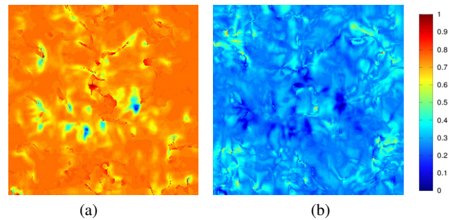
Figure 7: Flow field distances (accumulated l^2 -norm): (a) distance for flow fields generated separately for each level; (b) distance for flow fields derived from previous levels.
