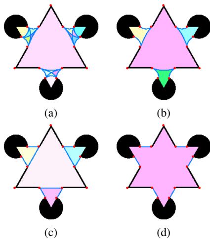
Figure 8: Influence of the parameters for our region closing algorithm: (a) Curved splines and low minimal area, (b) Curved splines and medium minimal area, (c) Straight splines and medium minimal area, (d) Straight splines and high minimal area.
