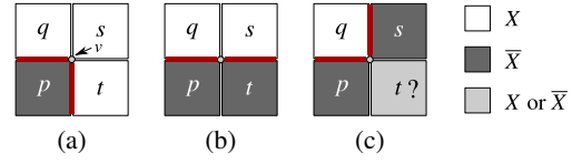
Figure 3: Adjacency relation between edges. Given 4 pixels p, q, s and t such that (p, q) \in \delta(X) , a single edge incident to the point v is in relation with (p, q) by \mathcal{R}_e . Thus: (p, q)\mathcal{R}_e(p, t) in case (a), (p, q)\mathcal{R}_e(t, s) in case (b), and (p, q)\mathcal{R}_e(s, q) in case (c) for any value of t .
