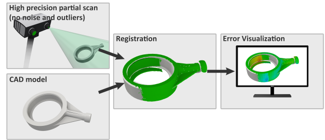
Figure 2: General overview over Nominal/Actual comparison. A part, manufactured from CAD, will be scanned and compared against its CAD by aligning the scanned data without noise and outliers onto the CAD data. Thus the deviation can be visualized.
