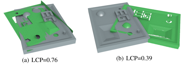
Figure 3: Problems of using a pure LCP-based approach. The configuration on the left has a relatively high LCP value. However, it will converge to an incorrect result after local refinement (ICP). In contrast, the result on the right converges to the global optimum in just 14 iterations, although the initial LCP value is rather low.
