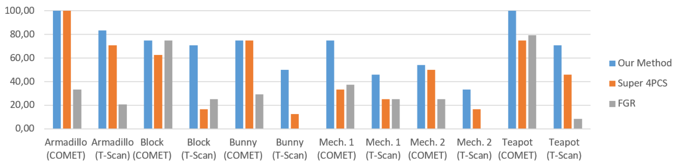
Figure 7: Registration success rate, measured as percentage of runs that achieved the correct result (the manually generated ground truth).
