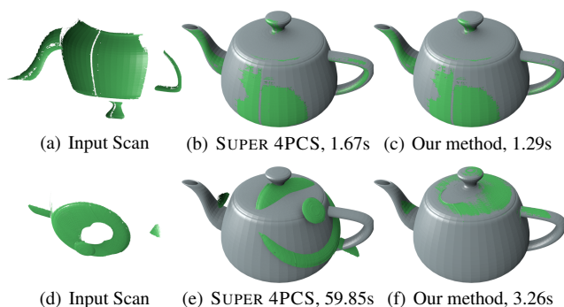
Figure 1: Registration of range images for Nominal/Actual comparison. Using existing building blocks, we propose a new method for global registration that achieves high success rates and fast registration, even for challenging input data. Our study uses real-world data from different high-end industrial scanners (top row: structured light scanner, bottom row: handheld laser scanner).
