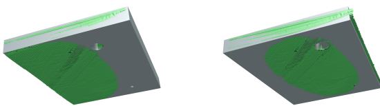
Figure 10: Problems arising from global deformations under rigid matching. Left: manually aligned ground truth. Right: alignment after local optimization via ICP.
