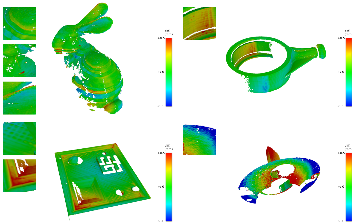
Figure 9: Visualization of different errors, originating from the 3D printing process. Data sets have been registered within a few seconds, using our method. Artifacts that can be seen include (from top left to bottom right): Ringing artifacts, originating from layering, along with small droplets of material and deviations from the desired thickness in steep regions (Bunny), small knobs from temporary congestion of the printing nozzle (Mech. Part 1), peaks on the thin surface, originating from the original support structure, plus slight bending on the edges of the model (Block), as well as strong bending of the base area of the model (Mech. Part 2).
