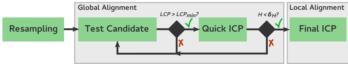
Figure 4: Our framework. Our global alignment algorithm includes a quick ICP stage in order to quickly evaluate whether a given candidate transformation should be regarded as an acceptable result. The quick ICP stage is only executed if the result already has a minimum quality.
